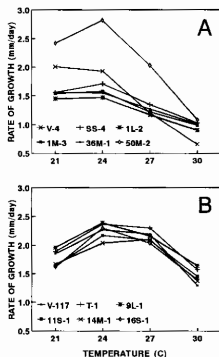
Fig. 1. Growth rate of (A) nondefoliating, and (B) defoliating isolates of Verticillium dahliae on potato dextrose agar at different temperatures in the dark.
