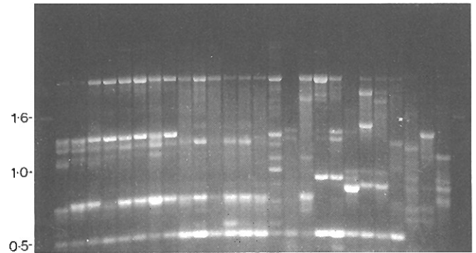
Fig 1. Random amplified polymorphic DNA analysis with primer P2 (5'-CACCGCCCCAAAATGGCCAC-3'). DNA was fractionated on a 2% agarose gel and stained with ethidium bromide. Numbers on the side are sizes in kilobase pairs. Lanes 1 and 28 are the 1-kb DNA ladder (GIBCO-BRL). Fusarium oxysporum f. sp. ciceris isolates (race and pathotype are given in parentheses): lane 2, 7932 (0, Y); lane 3, 7982 (0, Y); lane 4, 8733 (0, Y); lane 5, 82108 (0, Y); lane 6, 1987-B (0, Y); lane 7, 9018(JG62) (0, Y); lane 8, 9018(PV1) (0, Y); lane 9, 90111 (0, Y); lane 10, 9020 (6, W); lane 11, 9023 (6, W); lane 12, 9035 (5, W); lane 13, 9164 (6, W); lane 14, 9166 (1A, W); lane 15, 9168 (1A, W); lane 16, 9198 (0, Y). F. o. melonis isolates: lane 17, FOM VAL; lane 18, 1168; lane 19, 1173; lane 20, 1176; lane 21, 1178; lane 22, 1225. F. o. niveum isolates: lane 23, 1167; lane 24, 8527. Lane 25, F. eumartii 8013; lane 26, F. solani 8017; and lane 27, Ascochyta rabiei 8503.
