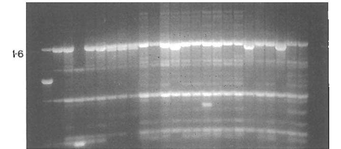
Fig 2. Random amplified polymorphic DNA analysis with primer KS (5'-CGAGGTCGACGGTATCG-3'). DNA was fractionated on a 2% agarose gel and stained with ethidium bromide. Number on the side is the size in kilobase pairs. Lanes 1 and 28 are the 1-kb DNA ladder (GIBCO-BRL). Fusarium oxysporum f. sp. ciceris isolates (race and pathotype are given in parentheses): lane 2, 7802 (0, Y); lane 3, 7952 (0, Y); lane 4, 8207 (0, Y); lane 5, 8250 (nonpathogenic); lane 6, 8310 (0, Y); lane 7, 8401 (0, Y); lane 8, 8012 (5, W); lane 9, 8408 (5, W); lane 10, 8257 (5, W); lane 11, 8317 (0, Y); lane 12, 8413 (0, Y); lane 13, 8415 (0, Y); lane 14, 8508 (5, W); lane 15, 82113 (0, Y); lane 16, 82115 (0, Y); lane 17, 8601 (0, Y); lane 18, 8602 (0, Y); lane 19, 8604 (0, Y); lane 20, 8901 (0, Y); lane 21, 8905 (6, W); lane 22, 8911 (0, Y); lane 23, 8912 (0, Y); lane 24, 8924 (6, W); lane 25, 8913 (0, Y); lane 26, 8914 (0, Y); and lane 27, control.
